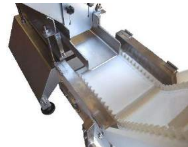
VIBRATORY FEEDER
