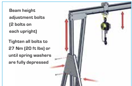
23. Decide on the height required (always using the lowest possible setting for the work in hand). Adjust the upright position on one A-Frame (a 2 man operation – one on the bolts and one on the upright) by removing 2 x upright securing bolts and moving the upright to the appropriate setting by lifting from the strut handle. Re-secure with bolts, nuts and washers (do not over tighten). Repeat the height adjustment at the opposite end.
