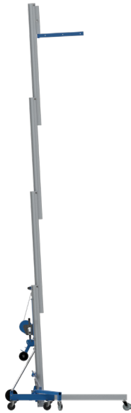
RML60 360kg Max load Added stabiliser legs
